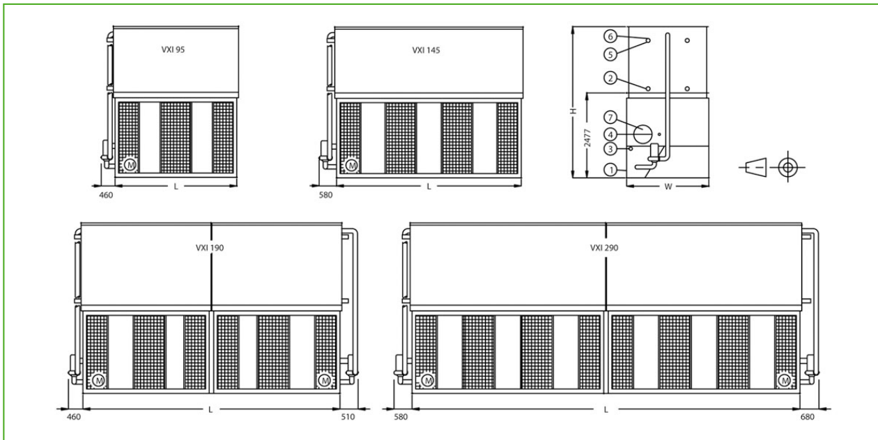
1. Drain ND50 (not shown); 2. Outlet Connection ND100; 3. Overflow ND80; 4. Make Up ND50; 5. Inlet Connection ND100; 6. Vent ND15; 7. Access Door.
