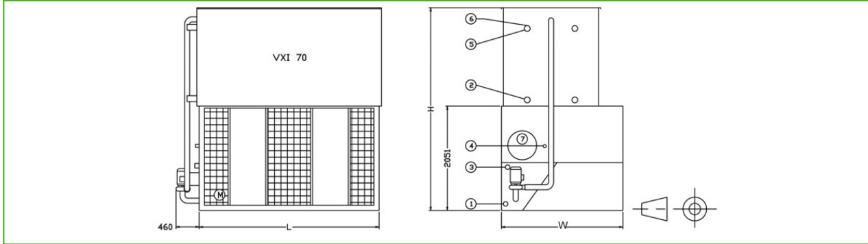
1. Drain ND50; 2. Outlet connection ND100; 3. Overflow ND80; 4. Make up ND50; Inlet connection ND100; 6. Vent ND15; 7. Access door.
